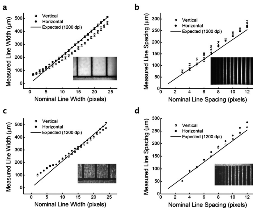
Fig. 2 Toner line widths printed onto photographic paper (vertical and horizontal), then transferred to brass substrates, were measured using wide-field microscopy and image analysis. (a) The horizontal line widths (filled circles) correlated well with the expected values of a 1200 dpi printer (solid line), while the vertical line widths (open squares) revealed a slightly rectangular pixel aspect ratio of the printer. (b) Toner line spacing was measured in a similar fashion, confirming the rectangular pixel aspect ratio. (c) Line widths and (d) spacing after thermal transfer to brass substrates. Insets show typical images from each analysis. Error bars represent standard deviations about mean values.
