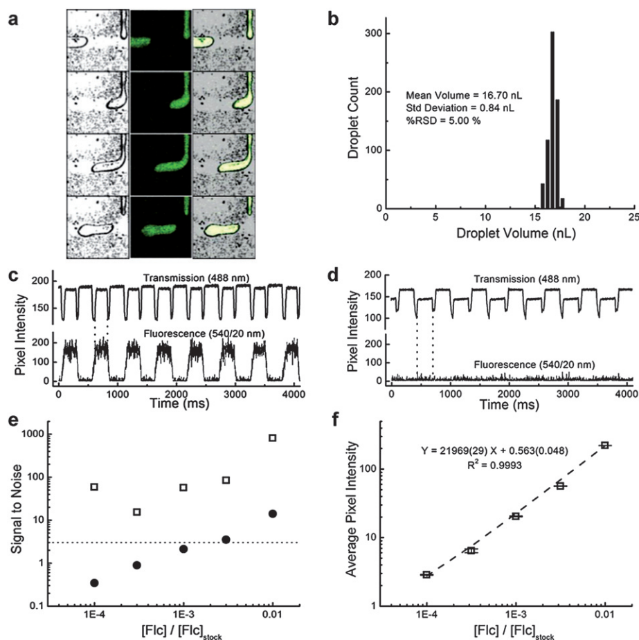
Fig. 4 Aqueous-in-oil droplet formation at a microfluidic T-junction. (a) Confocal transmission (left), fluorescence (middle), and combined (right) images as acquired during aqueous fluorescein droplet formation in silicone oil. (b) Droplets were monodisperse, with an average volume of 16.70 \pm 0.84 nL ( \pm \sigma ). (c) Correlation of transmission and fluorescence intensities allowed spatial and temporal lock-in-detection due to the 'sample chopping' effect of the droplets, even at (d) fluorescein concentrations below the LOD. (e) Signal-to-noise enhancements up to \sim 800 -fold were possible using lock-in spatial filtering (open squares), compared to unprocessed data (filled circles). Three of the five concentrations were undetectable (below the 3\sigma dotted line) until the data was processed. (f) Processed signal was linear over several orders of magnitude of concentration. Error bars represent standard deviations about mean values.
