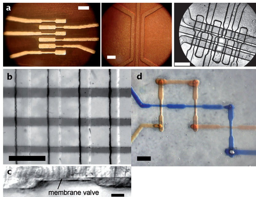
Fig. 3 Multilayer PDMS devices were fabricated using toner transfer masking (TTM) and multilayer soft lithography (MLS). (a) Wide-field images of two brass masters and the final device made with micro-pneumatic valves using MLS (left: pneumatic master, middle: fluidic master, right: final device). Image shows the fourth valve from left during actuation. (b) Image of assembled crossing PDMS valve structures, with air in the pneumatic channels (lower) and dye solution in the fluidic channels (upper). (c) Image of a sliced cross-section of a PDMS valve from (b), showing the membrane thickness of 26.6 \pm 0.7 \mu\text{m} ( \pm\sigma ) above a pneumatic actuation channel of 74.0 \pm 1.1 \mu\text{m} depth and \sim 560 \mu\text{m} width. (d) Image of crossing channels in a three-dimensional channel network, including vias with average volume of 2.5 \pm 0.6 \text{ nL} , made using TTM and MLS. Scale bars are 1 mm in (a), (b), and (d); 100 \mu\text{m} in (c).
