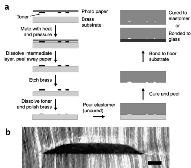
Fig. 1 Toner transfer masking (TTM) process for rapid, inexpensive, and cleanroom-free fabrication of microfluidic devices. (a) Illustration of the simple fabrication process in which masters are etched from brass then used to mold poly(dimethylsiloxane) (PDMS) microfluidic chips. The turnaround time for master fabrication ( \sim 1\text{--}2 h) as well as device molding ( \sim 1 h), dominated by the brass etching and polymer curing times, is typically around 2–3 hours. (b) An optical image of a sliced cross-section of a PDMS device, fabricated by TTM, reveals the channel cross-section to be trapezoidal, with tapered side walls that are faintly sigmoidal. Scale bar is 100\ \mu\text{m} .
